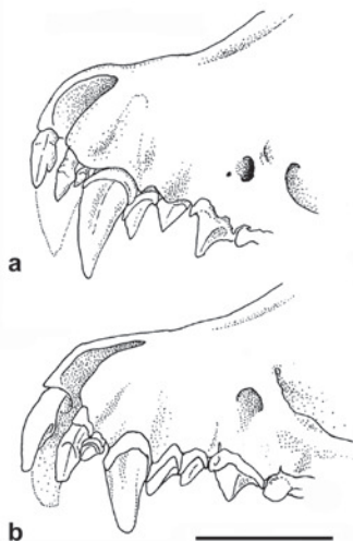
Fig. 29. Rostral and canine shape in a) Phoniscus jagorii and b) similar size Kerivoula ( K. kachinensis ) (scale bar 3 mm).
