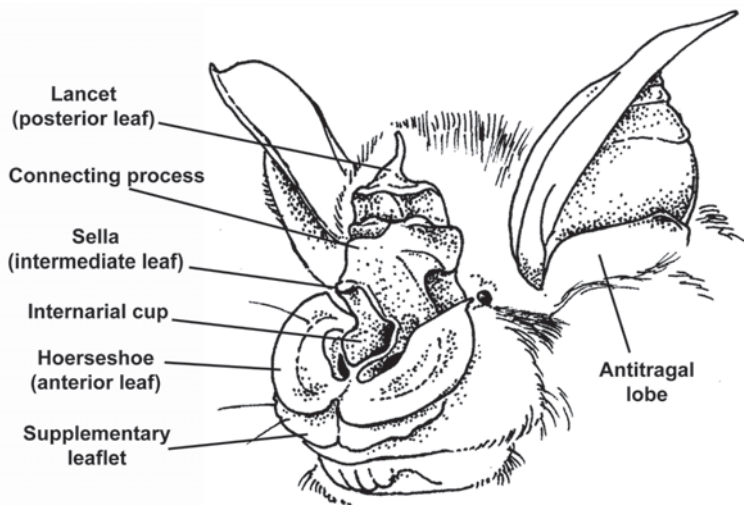
Fig. 17. Head of Rhinolophus chaseni , demonstrating details of noseleaf structure.
