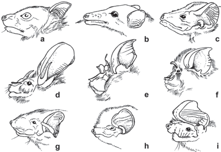
Fig. 8. Variation in the shape of muzzle and ears in Indo-Chinese Chiroptera: a) Pteropodidae ( Cynopterus ); b) Pteropodidae ( Macroglossus ); c) Emballonuridae ( Taphozous ); d) Megadermatidae ( Megaderma ); e) Rhinolophidae ( Rhinolophus ); f) Hipposideridae ( Hipposideros ); g) Vespertilionidae ( Scotophilus ); h) Miniopteridae ( Miniopterus ); i) Molossidae ( Chaerephon ).
