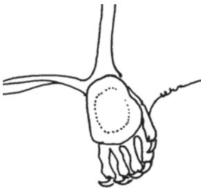
Fig. 36. Left hind foot of Eudiscopus denticulus , showing adhesive disc (ventral view).
