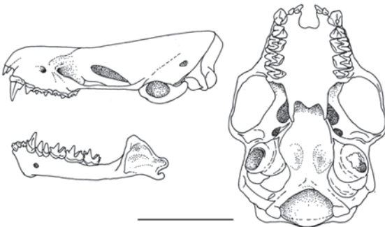
Fig. 64. Skull of Tylonycteris pachypus ZMMU S-172658 (scale bar 5 mm).
