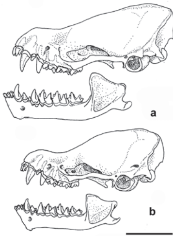
Fig. 34. Skull lateral views of the two Myotis montivagus morphotypes: a) large form, based on specimen from Vu Quang, and b) typical form based on specimen from Lao Cai.
