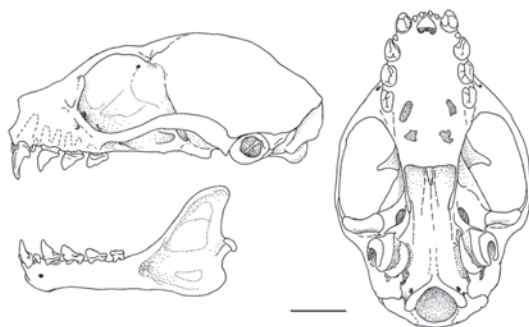
Fig. 41. Skull of Megaerops niphanae ZMMU S-168329 (scale bar 5 mm).
