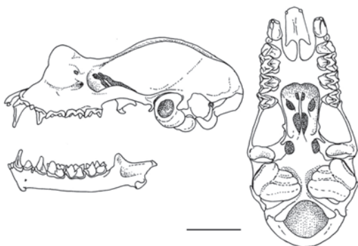
Fig. 48. Skull of Rhinolophus shameli ZMMU S-168305 (scale bar 5 mm).
