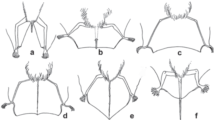
Fig. 9. Structure of the interfemoral membrane (uropatagium) in Vietnamese bats (dorsal view). a) Pteropodidae ( Eonycteris ); b) Emballonuridae ( Taphozous ); c) Megadermatidae ( Megaderma ); d) Rhinolophidae ( Rhinolophus ); e) Vespertilionidae ( Scotomanes ); f) Molossidae ( Chaerephon ).
